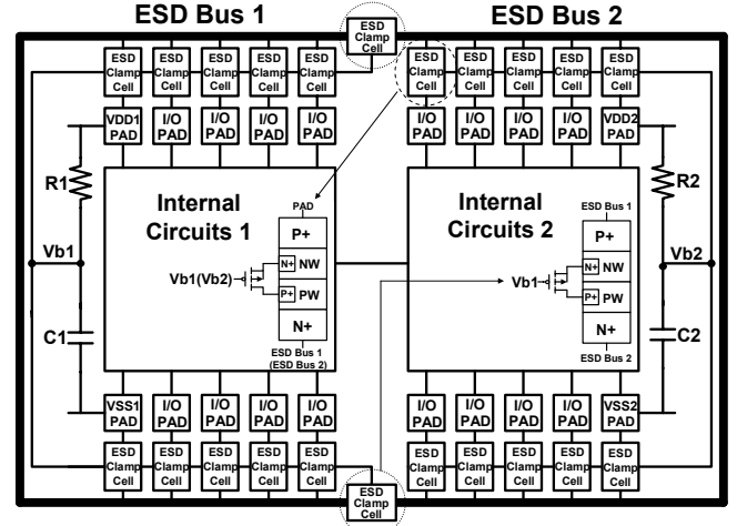
Fig. 5 The ESD protection scheme realized with the initial-on SCR design and ESD buses for the chip with separated power domains.
