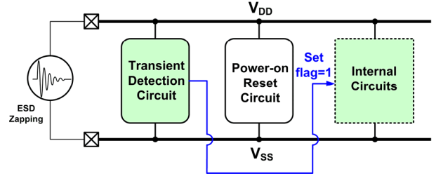
Fig. 5. Hardware/firmware operation during the system-level ESD stress.
