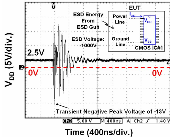
Fig. 2. Measured V_{\text{DD}} transient waveform on the CMOS ICs inside EUT with the abn ESD voltage of -1000V zapping on the HCP.
