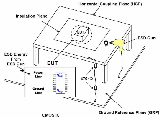
Fig. 1. Measurement setup of the system-level ESD test with indirect contact-discharge test mode.
