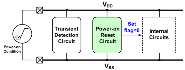
Fig. 4. Hardware/firmware operation during power-on reset condition.
