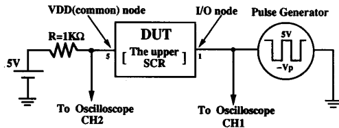
Fig. 6. The experimental setup to measure the ac triggering voltage of the fabricated ESD protection circuits.
