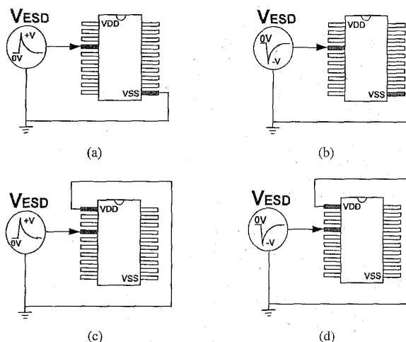
Fig. 1. A schematic diagram to show the four modes of ESD stresses: (a) PS-mode, (b) NS-mode, (c) PD-mode, and (d) ND-mode.
