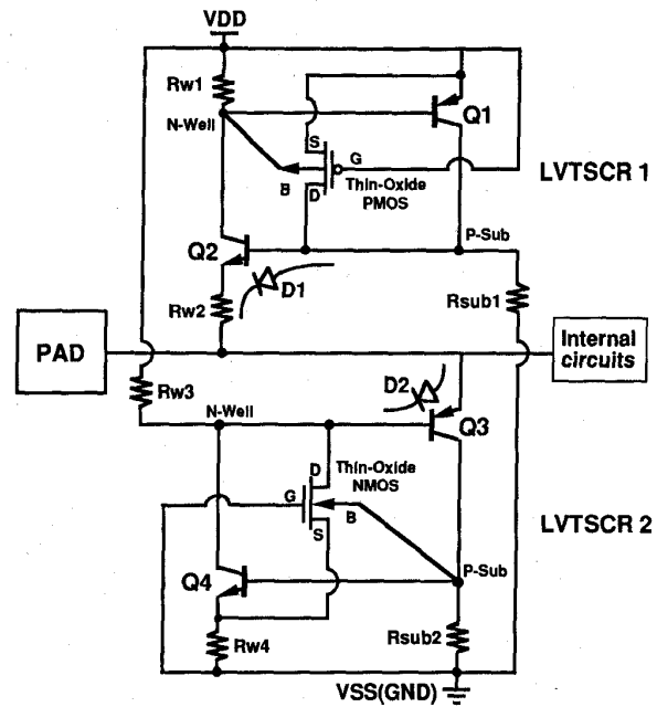
Fig. 3. The complementary-LVTSCR ESD protection circuit.
