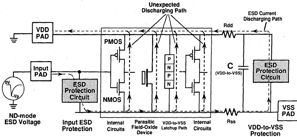
Fig. 2. A schematic diagram to show the unexpected discharging paths in the internal circuits but beyond the ESD protection circuits of CMOS IC's due to ND-mode ESD stress on the input pad.
