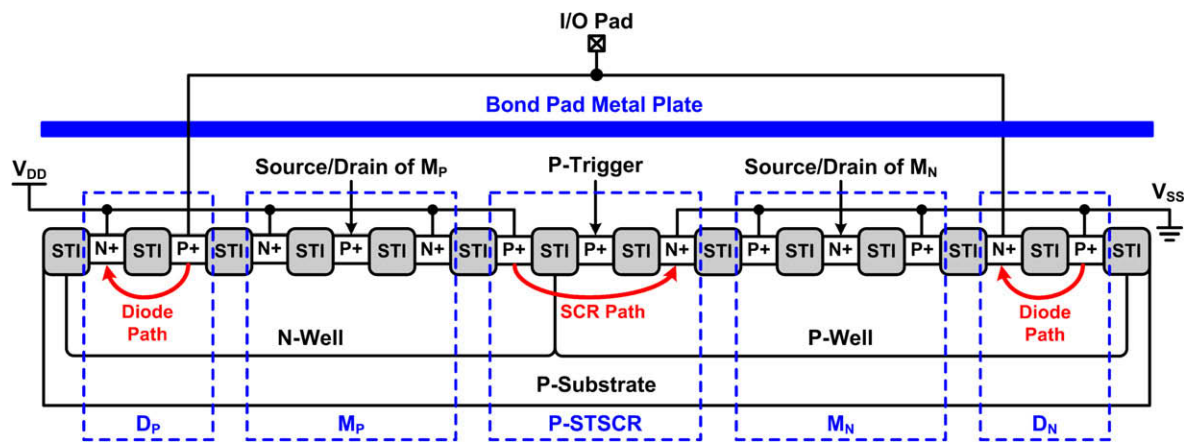
Fig. 14. Cross-sectional view of the ESD protection devices under the bond pad.
