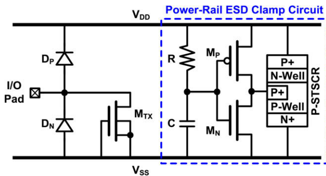
Fig. 10. Transmitter NMOS emulator used as a test circuit to verify the effectiveness of the proposed ESD protection scheme in a transmitter (double diodes and active power-rail ESD clamp circuit).
