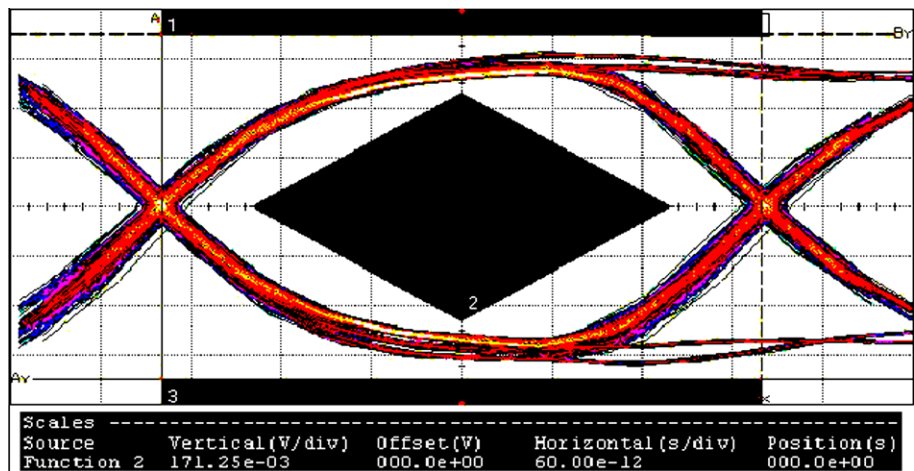
Fig. 15. Measured eye diagram of the 2.5-Gb/s high-speed I/O interface circuit fabricated in a 130-nm CMOS process.
