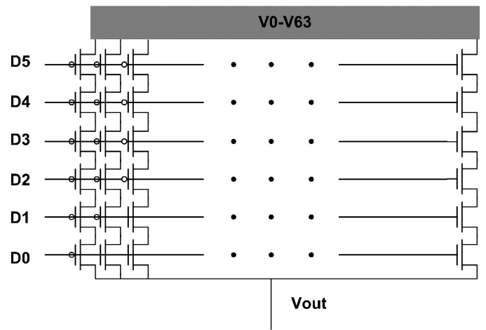
FIGURE 3 — A 6-bit R-string DAC with switch array decoding (Ref. 9).
