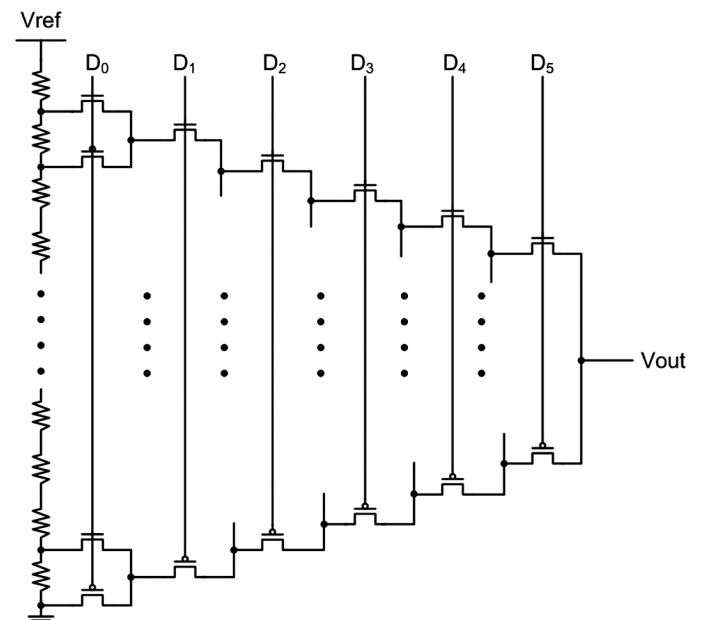
FIGURE 4 — A 6-bit R-string DAC with binary-tree decoding (Ref. 10).
