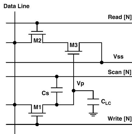
Fig. 1. Dynamic digital MIP circuit realized with three n-type TFTs for one bit operation [2].
