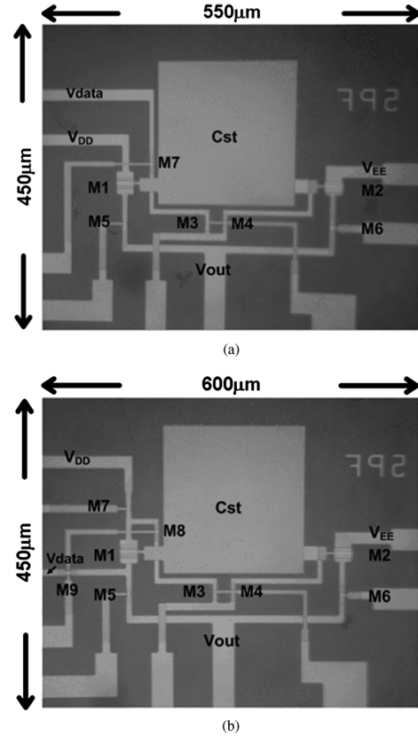
Fig. 8. Die photo of the proposed. (a) Analog memory cell I. (b) Analog memory cell II, fabricated in a 3\text{-}\mu\text{m} LTPS process.
