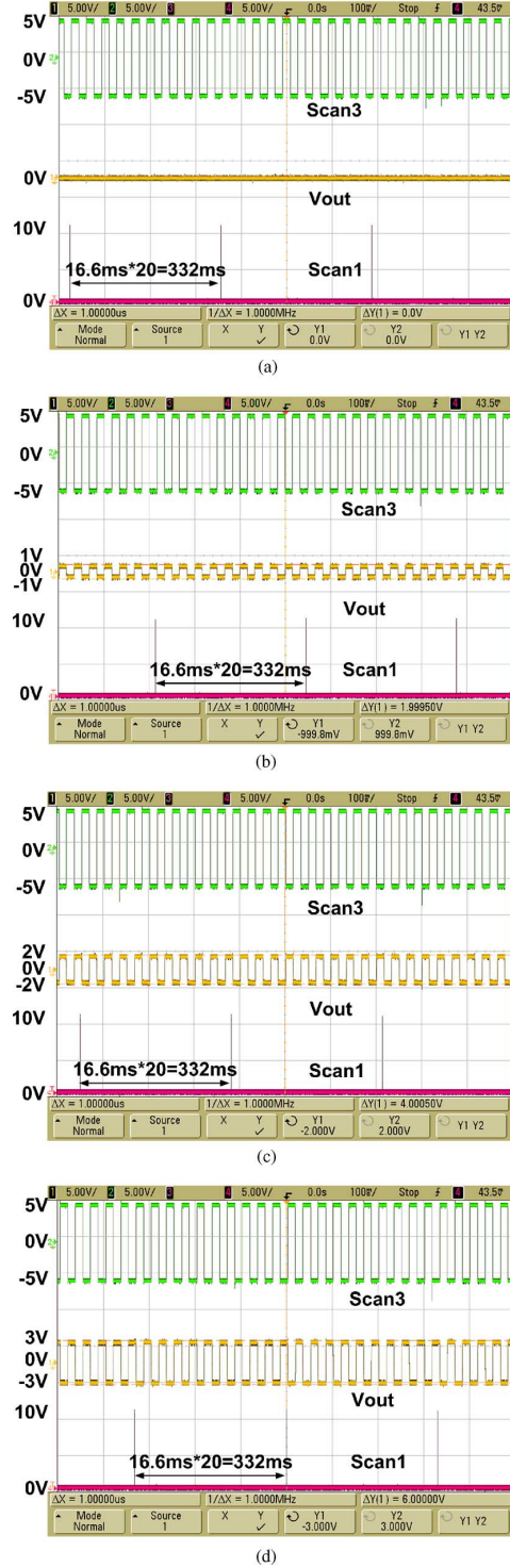
Fig. 9. Measured results of analog memory cell I with: (a) V_{data} = 1 V; (b) V_{data} = 2 V; (c) V_{data} = 3 V; and (d) V_{data} = 4 V in 20-frame time ( 16.6 \text{ ms} * 20 = 332 \text{ ms} ) per Scan1 pulse.
