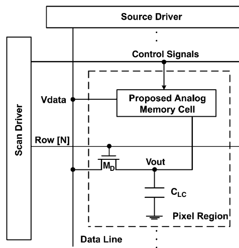
Fig. 2. Block diagram of the proposed analog memory cell in a conventional pixel.
