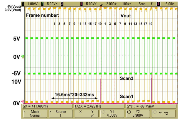
Fig. 13. The enlarged plot for V_{out} as 1 V/scale in Fig. 12(d) when V_{data} is 4 V. The entire V_{out} waveform is contained to show the output symmetry.
