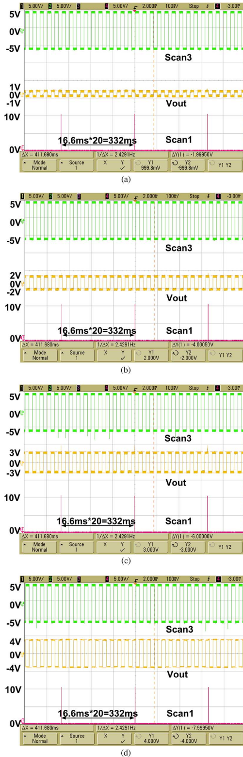
Fig. 12. Measured results of analog memory cell II with: (a) V_{data} = 1 V; (b) V_{data} = 2 V; (c) V_{data} = 3 V; and (d) V_{data} = 4 V in t20-frame time ( 16.6 \text{ ms} \times 20 = 332 \text{ ms} ) per Scan1 pulse.
