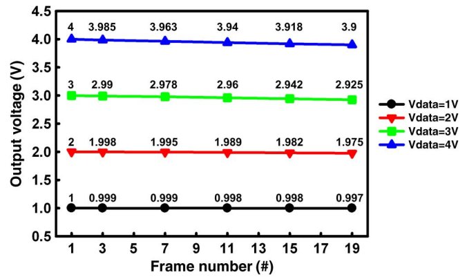
Fig. 14. The output voltage under different frame numbers with V_{data} of 1, 2, 3, and 4 V, respectively, in the proposed analog memory cell II for the positive output voltage.
