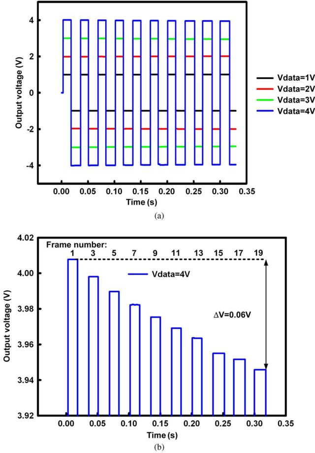
Fig. 6. Simulation results of the output ( V_{out} ) in the proposed analog memory cell II under: (a) V_{data} of 1 V, 2 V, 3 V, and 4 V in 20-frame time per Scan1 pulse, and (b) the partial enlarged plot when V_{data} is 4 V.
