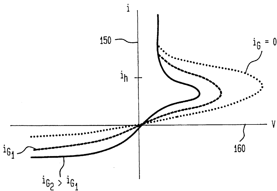
FIG. 1C (PRIOR ART)
