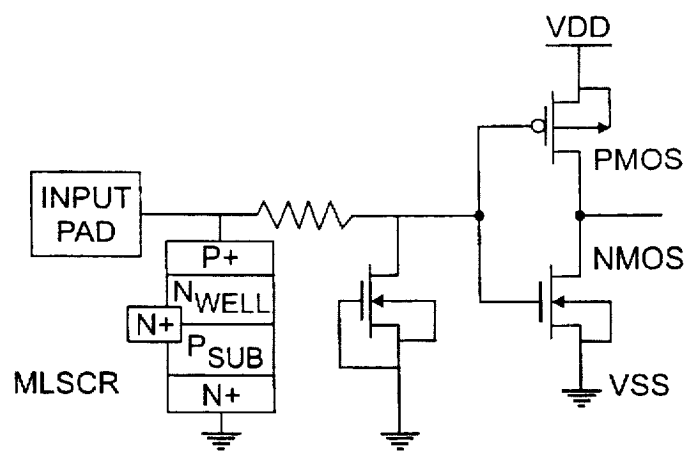
FIG. 2C PRIOR ART
