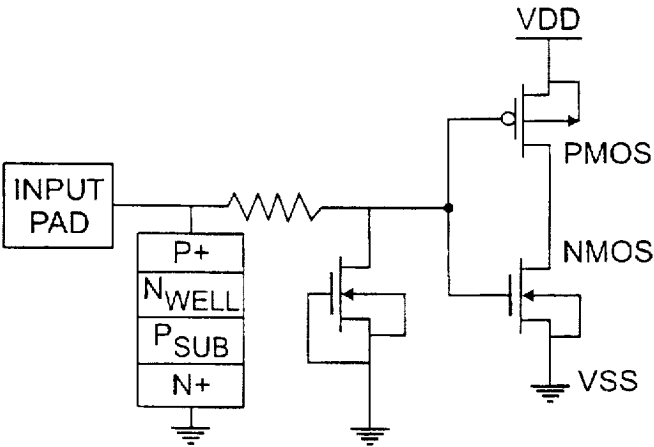
FIG. 1C PRIOR ART
