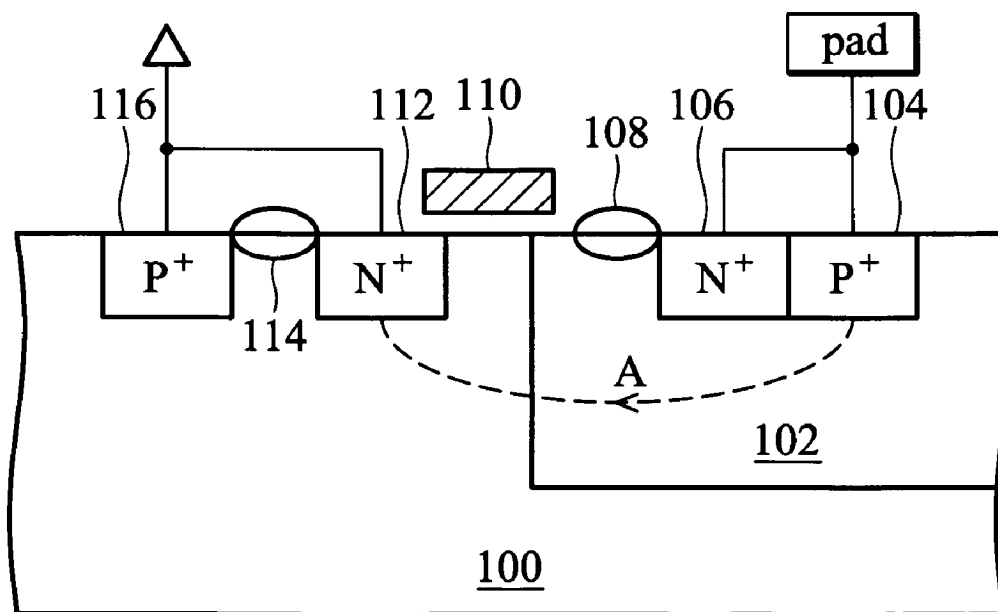
FIG. 2 (RELATED ART)
