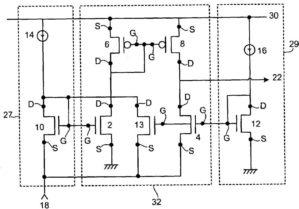
Fig.3(prior art)
