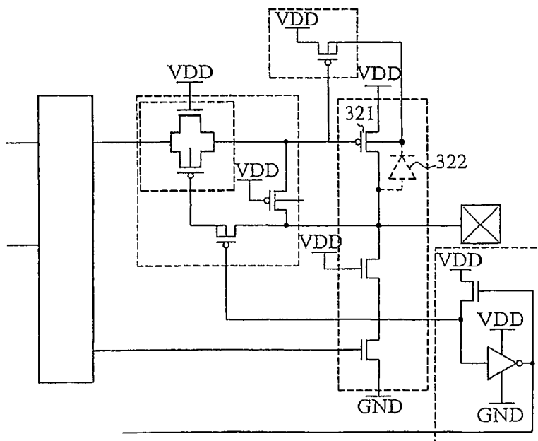
Fig. 6 (PRIOR ART)
