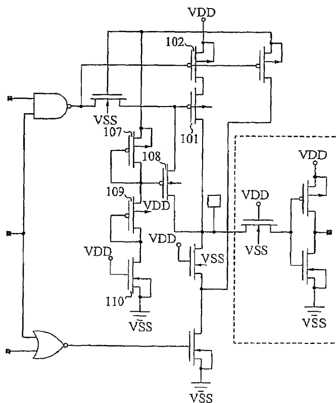
Fig. 2 (PRIOR ART)
